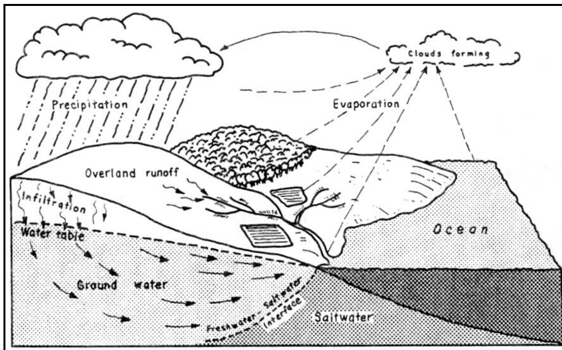
Figure D-1 The Hydrologic cycle (USEPA Seminar Publication)
